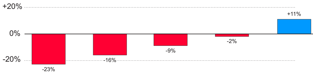
Figure 8. Projected changes in modeled natural flows (without storage or diversions) of the Colorado River near the Colorado-Utah state line, compared with historical values for 1950-2005. Results from five climate model/emission scenario combinations, chosen to approximate the range of the middle 80 percent of 112 such combinations from one database. Source: AECOM. 93
