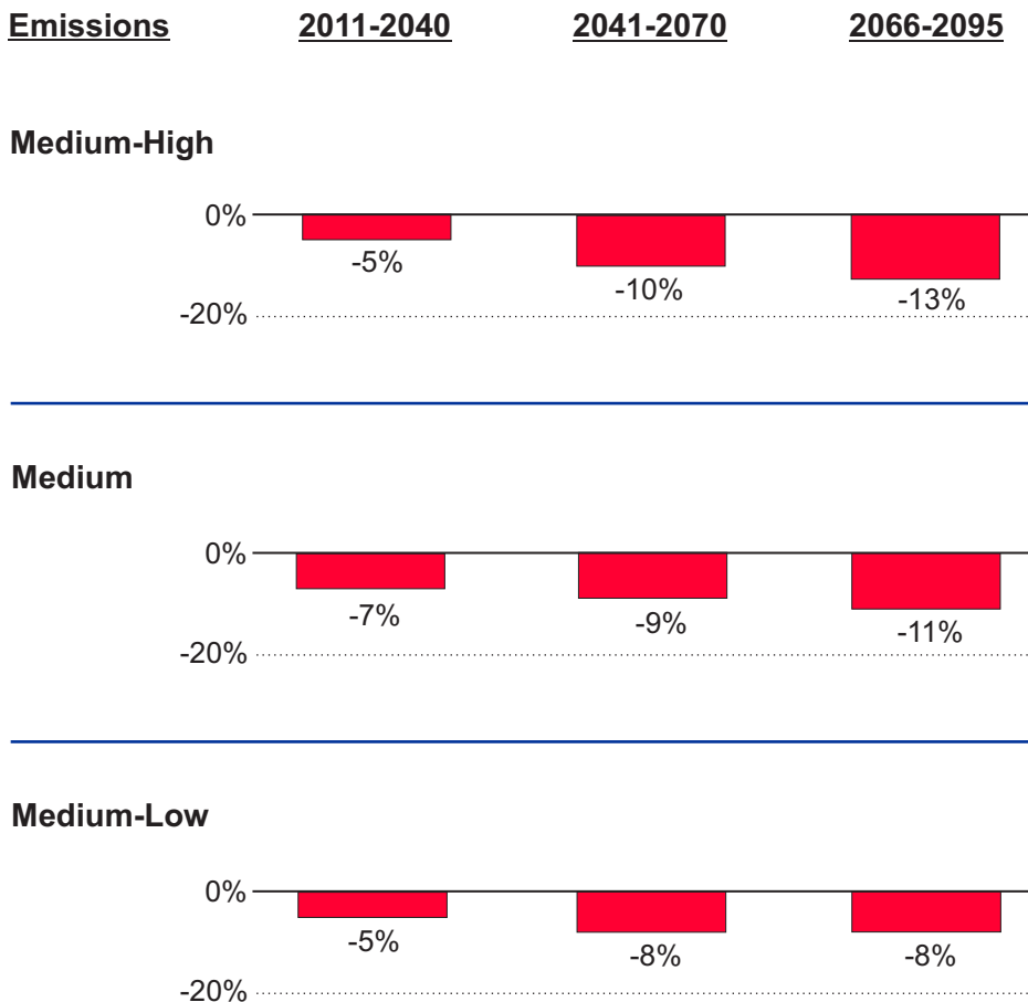
Figure 7. Projected change in Colorado River natural flows (without storage or diversions) at Lees Ferry, Arizona, showing averages of projections for each of three alternative scenarios of future heat-trapping emissions, compared to 1950 through 1999 historic flows. Total projections include 36 for the medium-high scenario, 39 for the medium, and 37 for the medium-low (see page 8). Despite the labels used here, the “medium” scenario has the highest level of emissions in the first time period (see Figure 4A on page 8); consistently across the projections, therefore, higher emissions are associated with greater flow reductions. As these projections are of modeled natural flow without storage or diversions, changes in water demands (see page 16) are not factored into these projections. Data source: U.S. Bureau of Reclamation. 90
